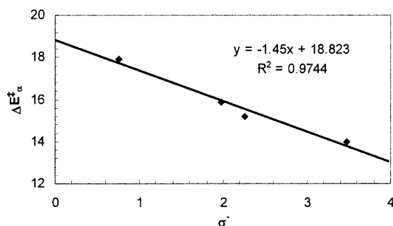
Figure 3. Transition-state energy barrier for \alpha -addition ( \Delta E_{\alpha}^{\ddagger} ) vs. Hammett constant \sigma^{-} .
